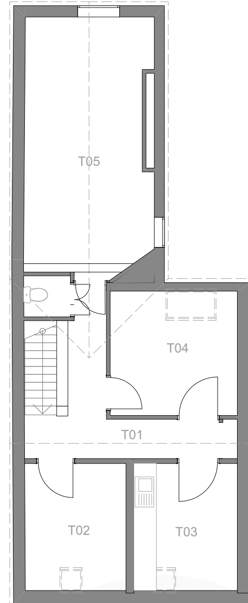
Third Floor Plan 1:100
