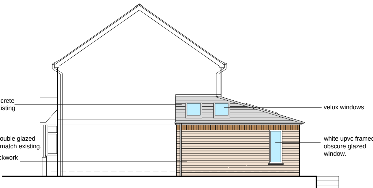
PROPOSED SIDE ELEVATION facing no.25
