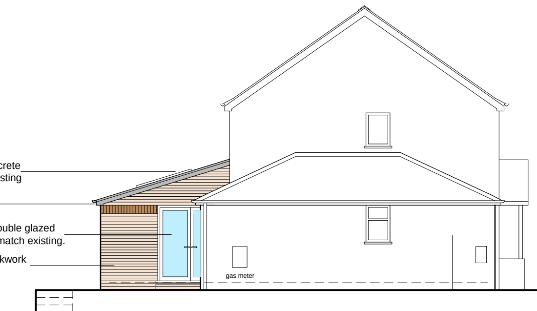
PROPOSED SIDE ELEVATION facing no.21
