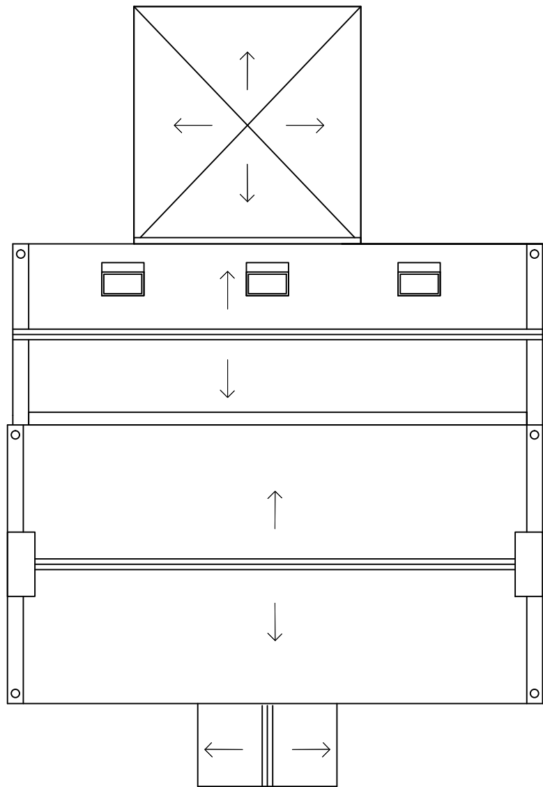
Roof Plan
