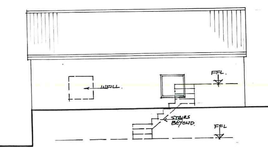
SIDE ELEVATION N.E. AS PROPOSED.
