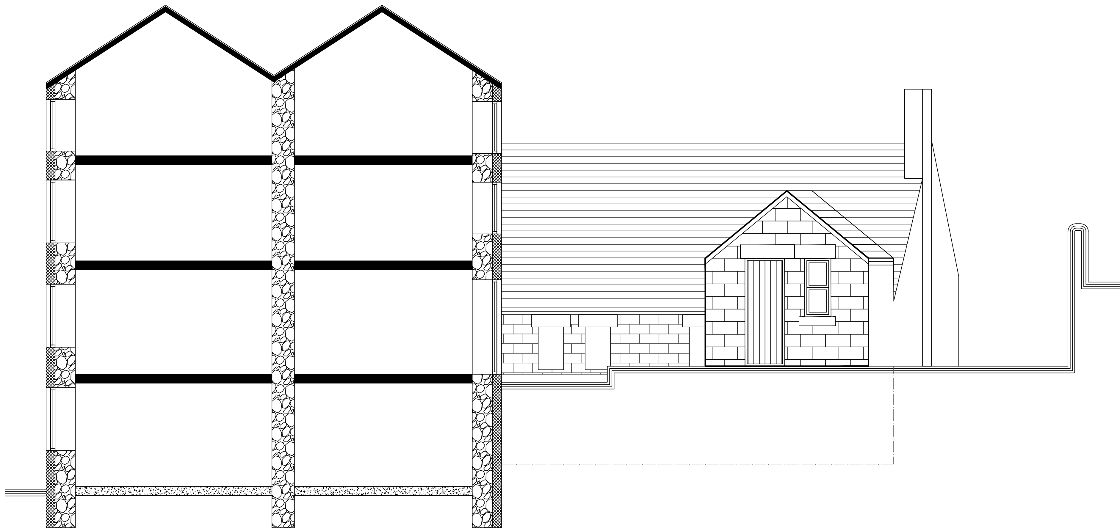
SECTIONAL BARN ELEVATION AS EXISTING 1:50 SECTIONAL SIDE ELEVATION AS EXISTING 1:50
