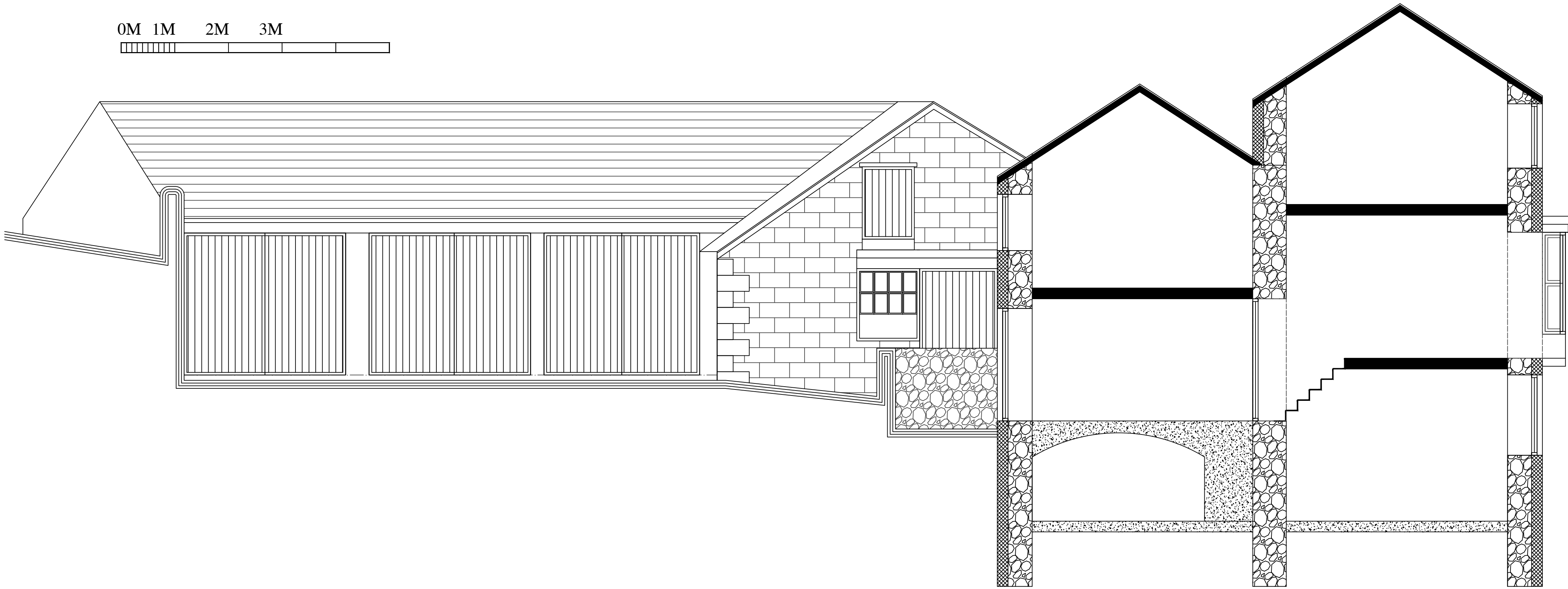
SECTIONAL BARN ELEVATION AS EXISTING 1:50 SECTIONAL SIDE ELEVATION AS EXISTING 1:50
