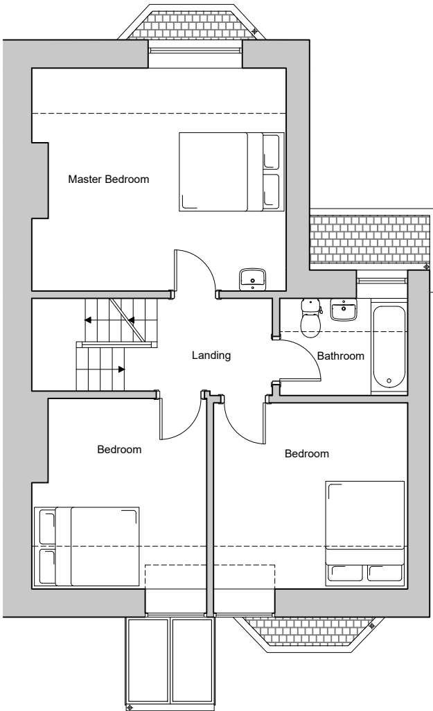
FIRST FLOOR PLAN: AS EXISTING 1:100
