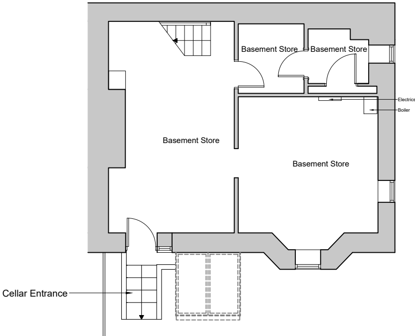
BASEMENT PLAN: AS EXISTING 1:100
