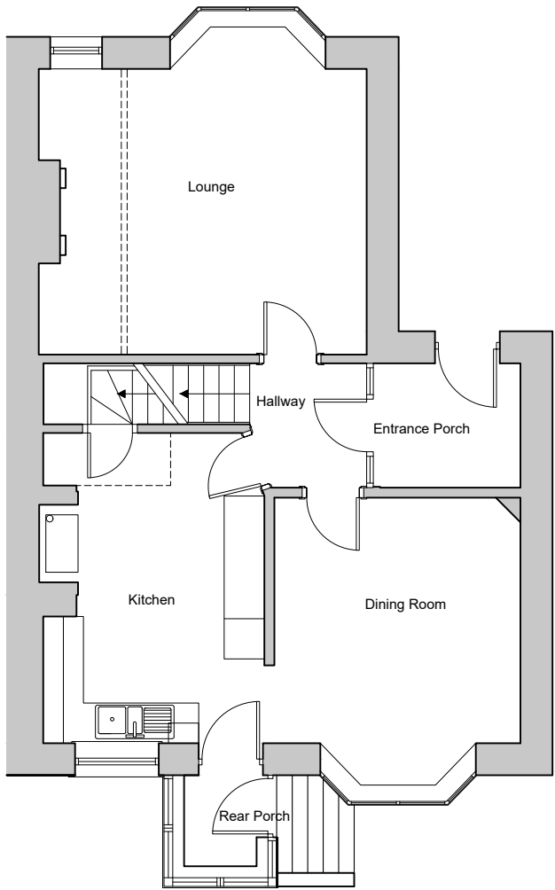
GROUND FLOOR PLAN: AS EXISTING 1:100
