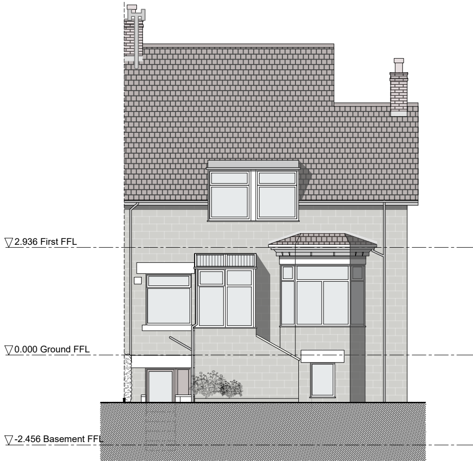
NORTH WEST ELEVATION: AS EXISTING 1:100
