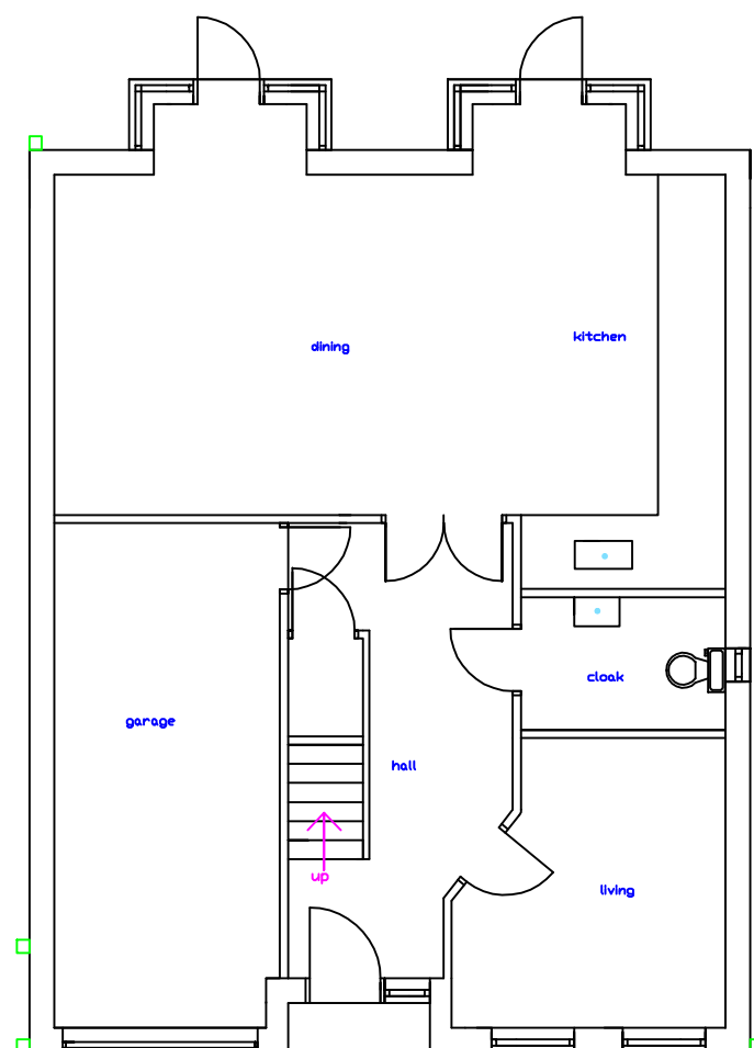
PROPOSED GROUND FLOOR 1: 100
