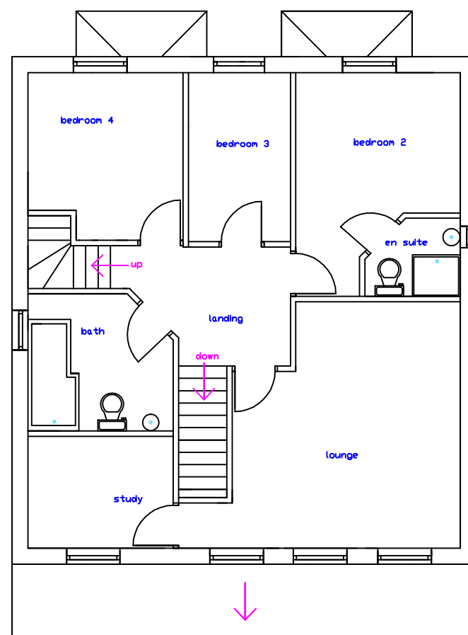
PROPOSED FIRST FLOOR 1: 100
