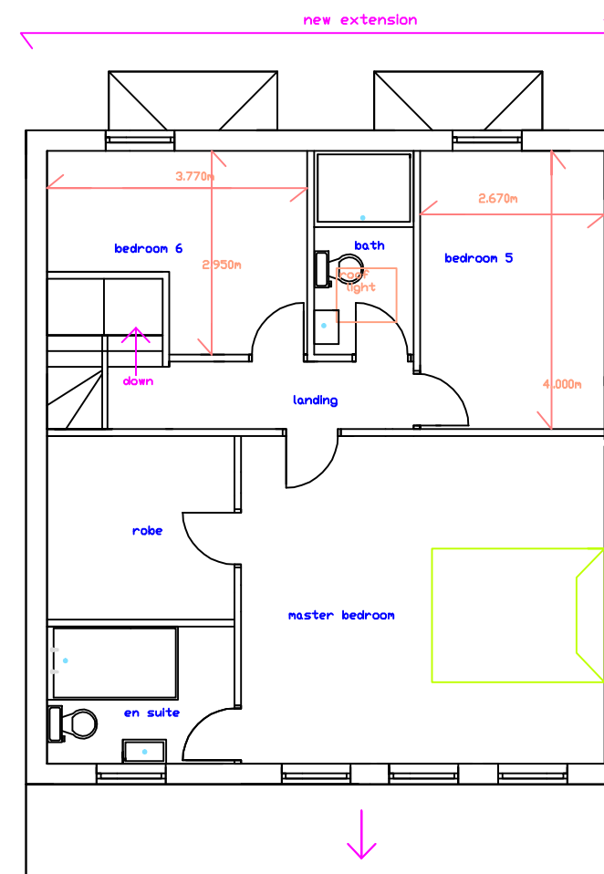
PROPOSED SECOND FLOOR 1: 100
