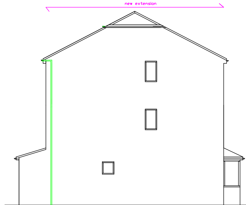
PROPOSED SIDE VIEW B 1: 100
