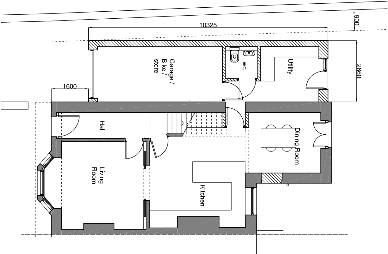
Ground Floor
