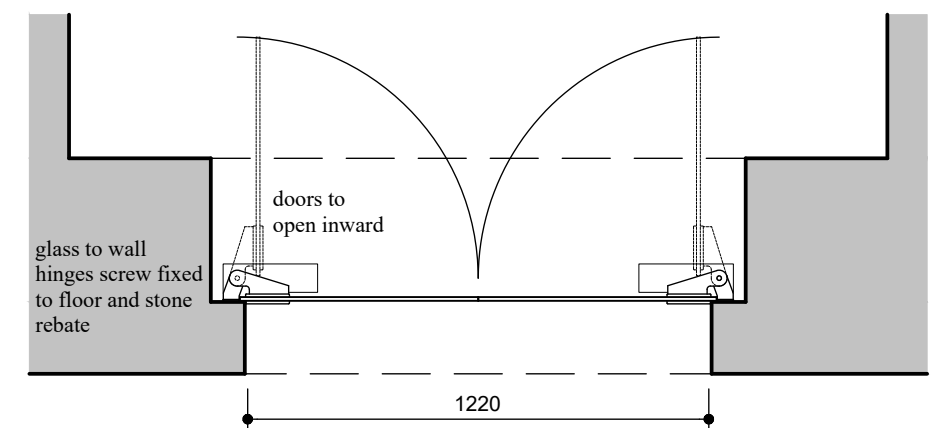
Front Door Detail
