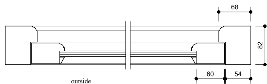
Casement Windows Details
