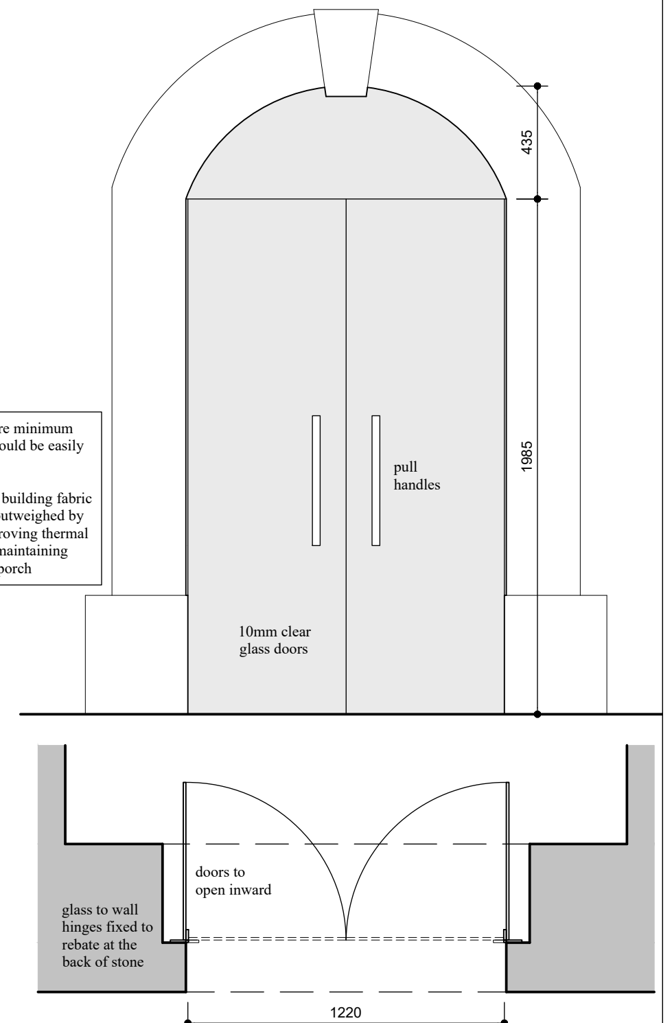
Front Door Detail
