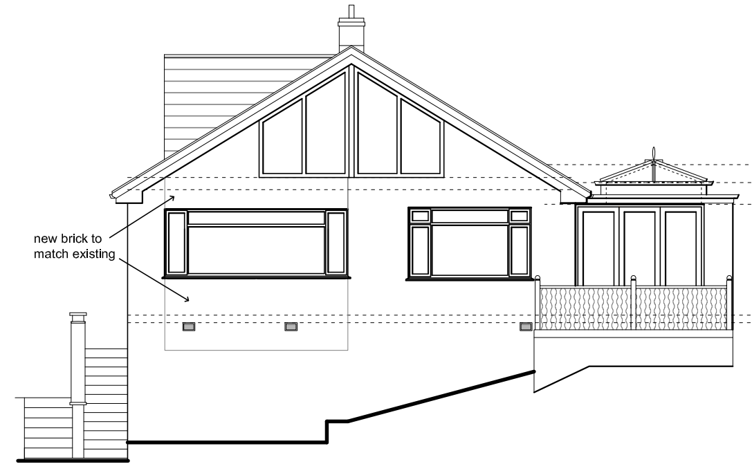
South Elevation
