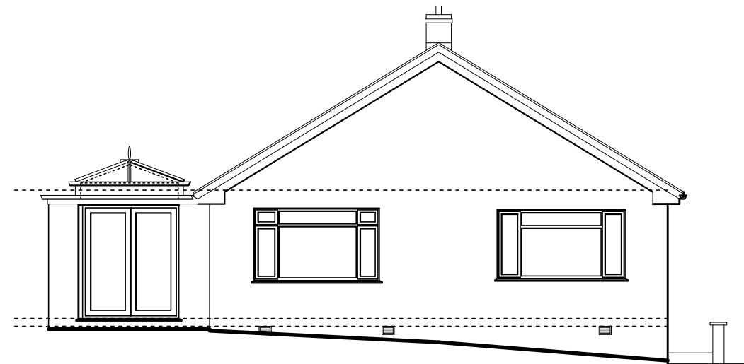
North Elevation
