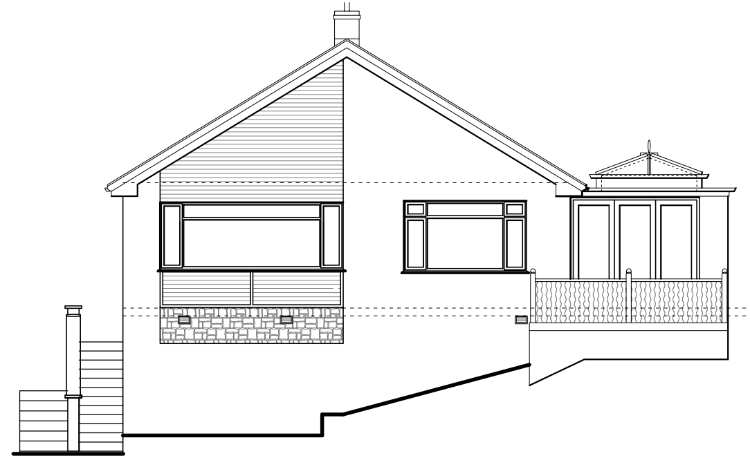
South Elevation
