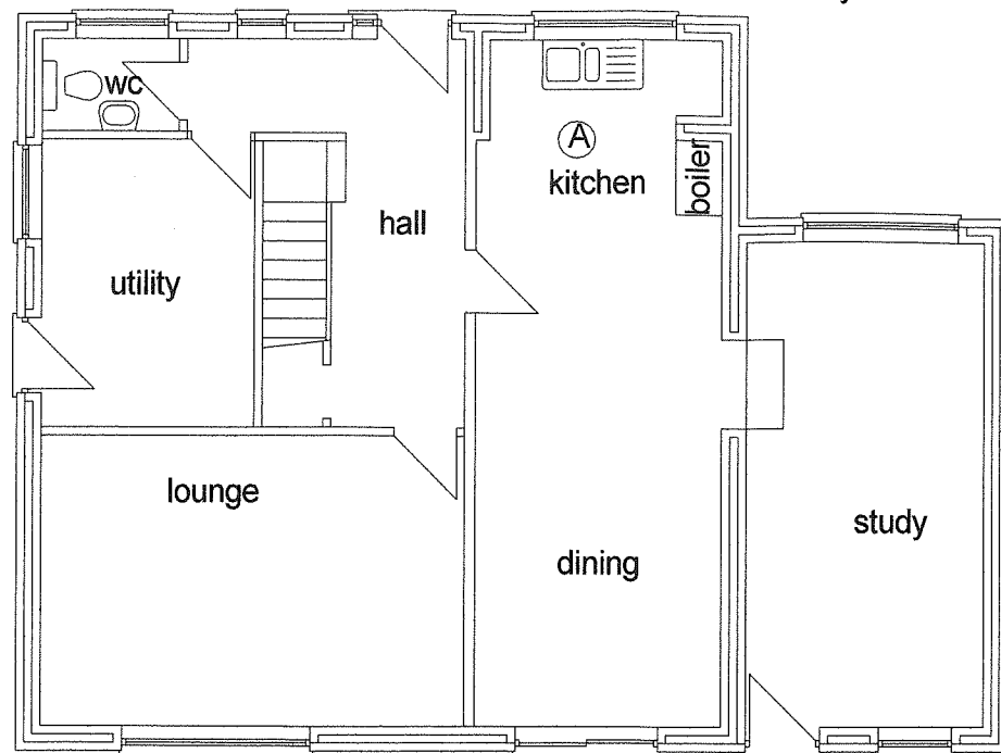
GROUND FLOOR Conservatory omitted
