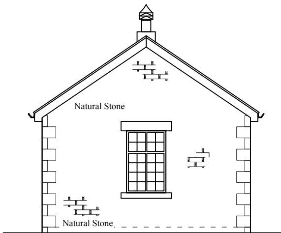
North (Side)
