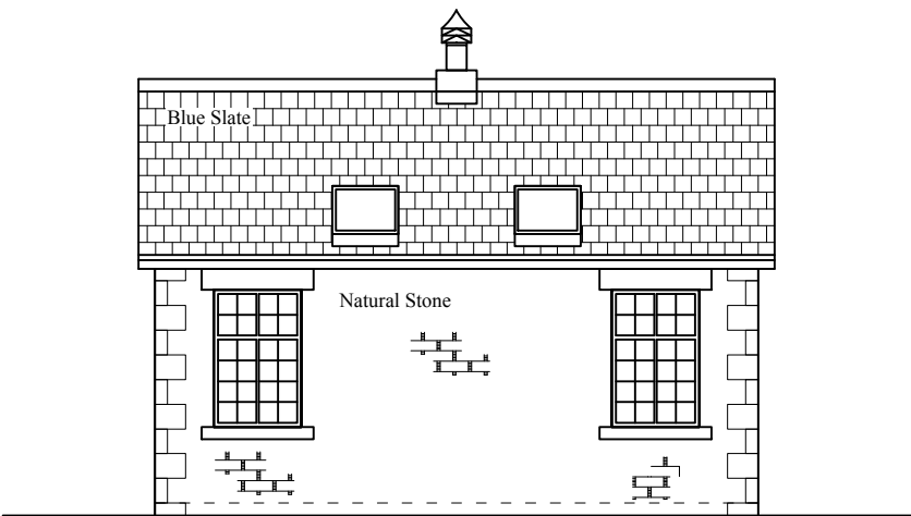
East (Rear)
