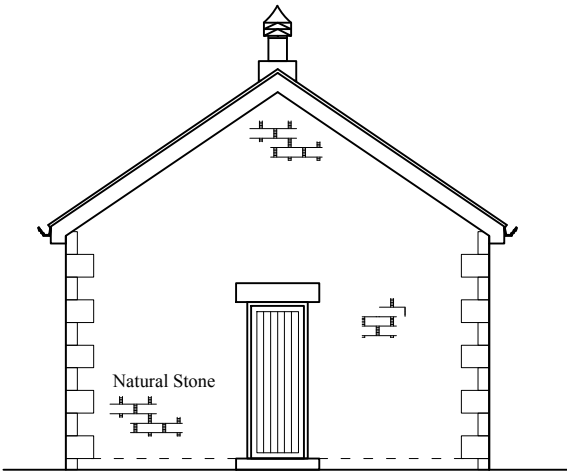
South (Side)
