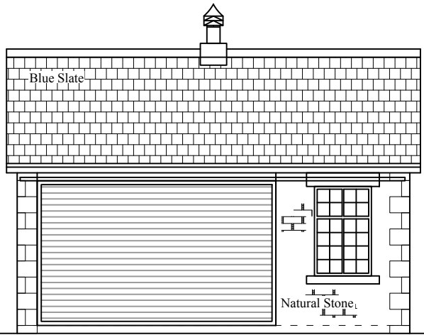
West (Front)
