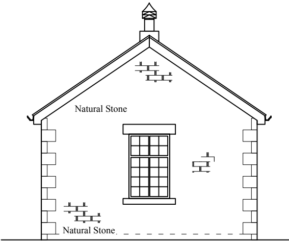
North (Side)
