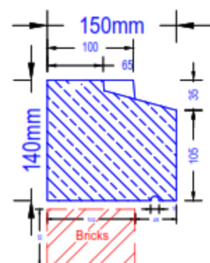
Cill Section Type C1
