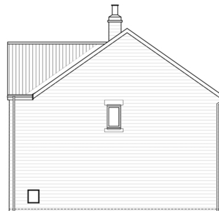
SIDE ELEVATIONS
