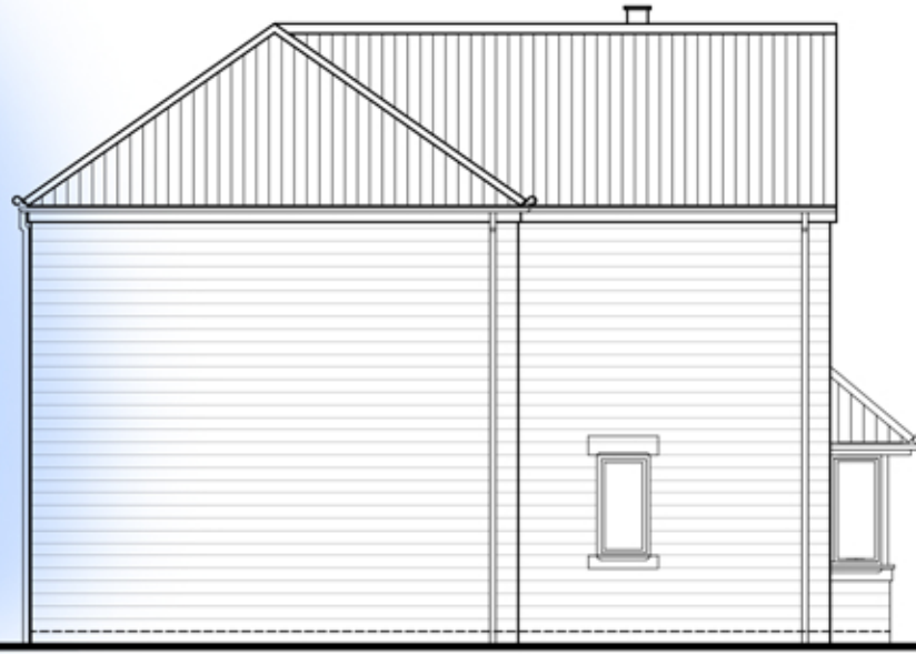
SIDE ELEVATION
