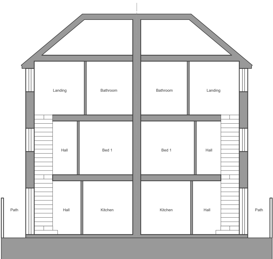
Indicative Section AA
