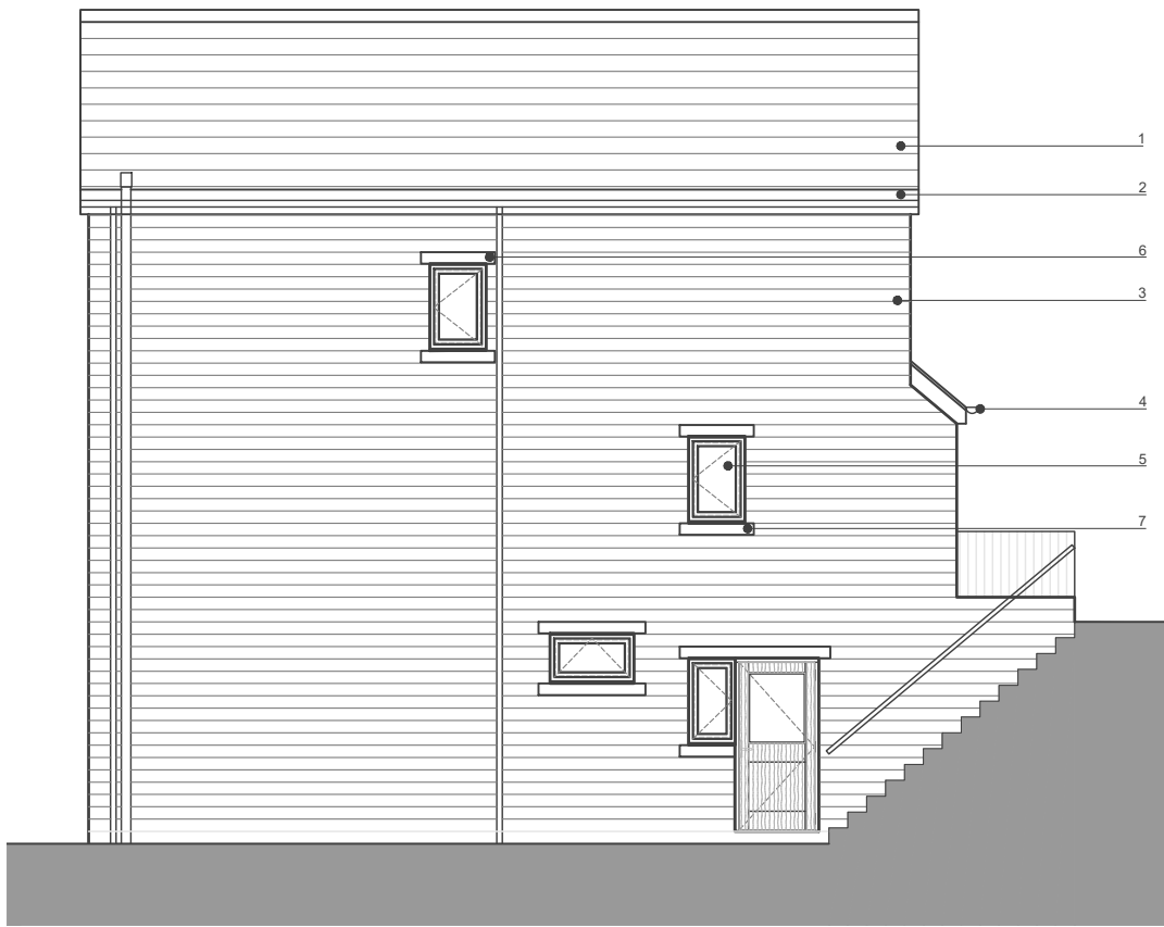
Side Elevation
