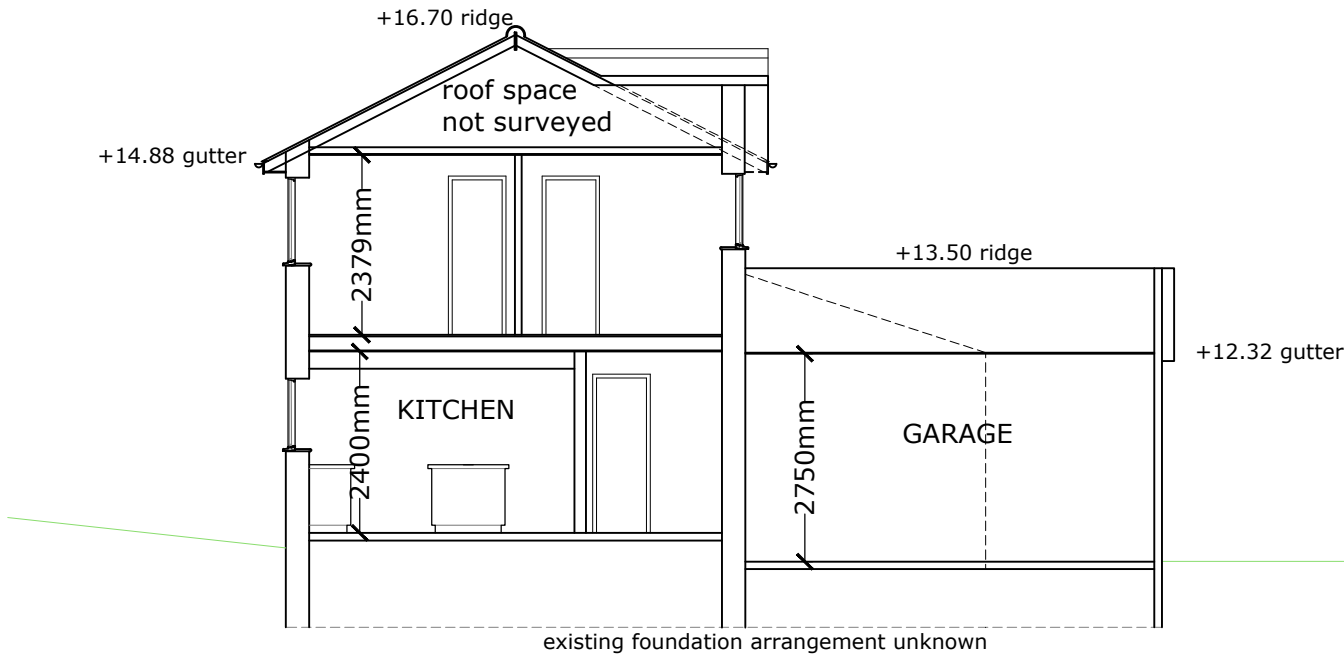
CROSS SECTION
