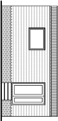
Front Elevation (north facing)
