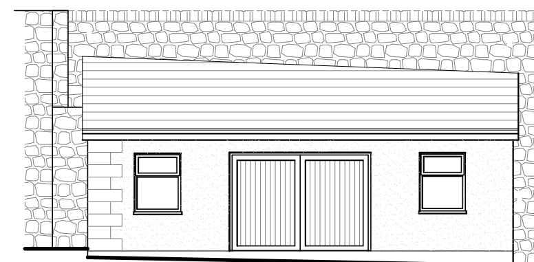
West Elevation
