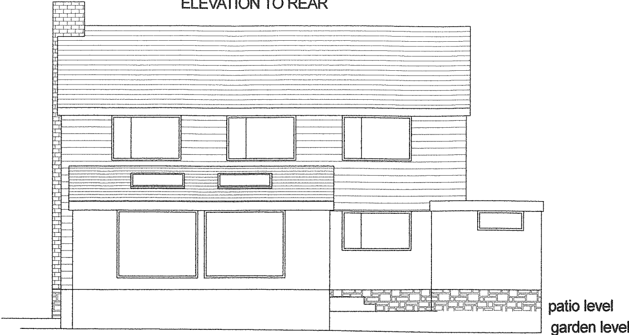
ELEVATION TO REAR
