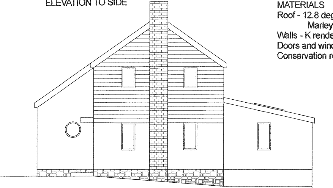
ELEVATION TO SIDE
