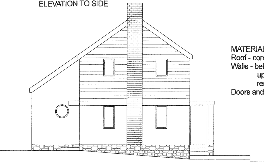
ELEVATION TO SIDE
