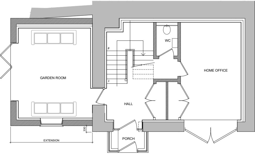
PROPOSED LOWER GROUND FLOOR PLAN 1:100
