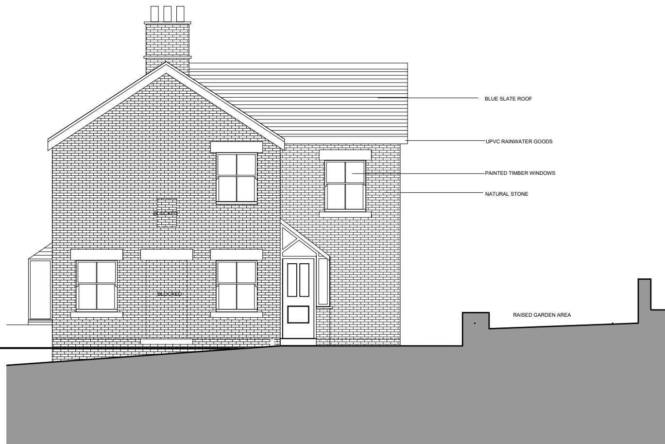
EXISTING WEST ELEVATION 1:100
