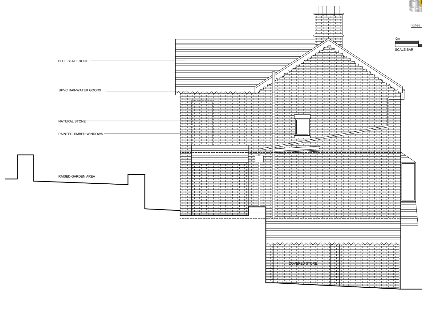
EXISTING WEST ELEVATION 1:100
