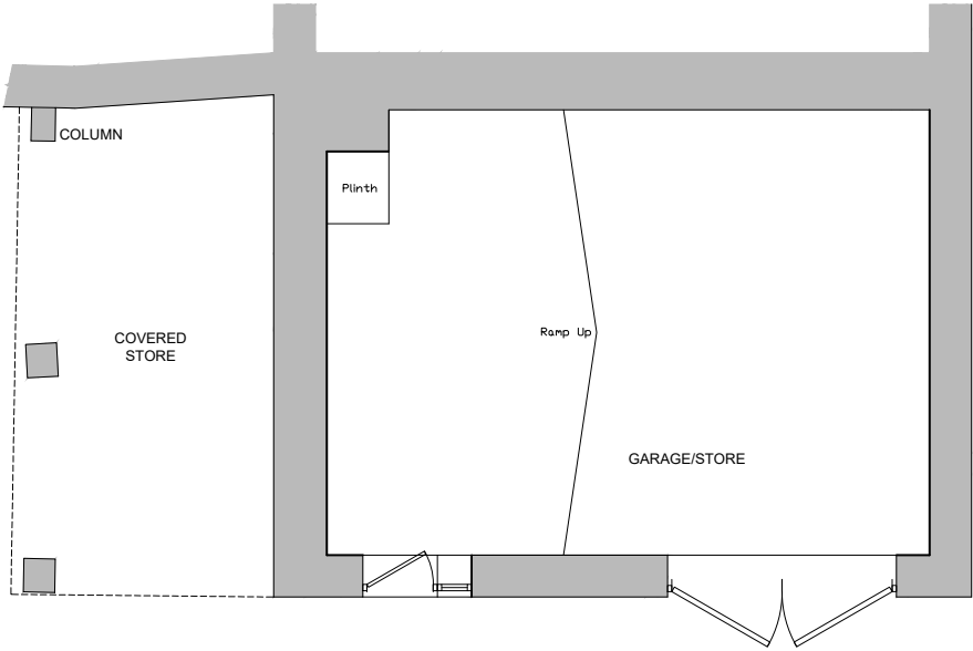
EXISTING LOWER GROUND FLOOR PLAN 1:100
