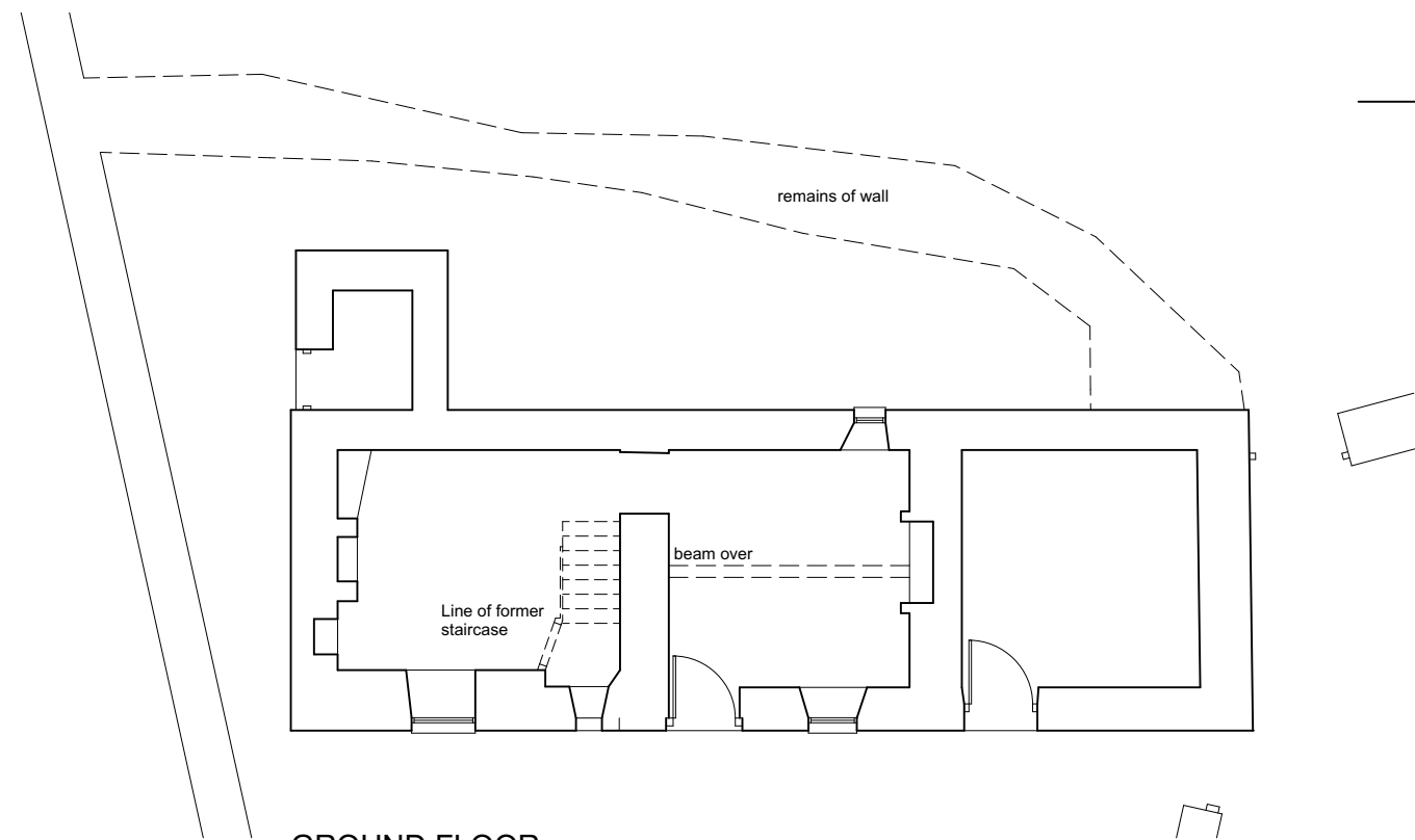
GROUND FLOOR
