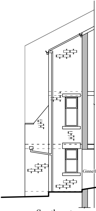
Southeast
