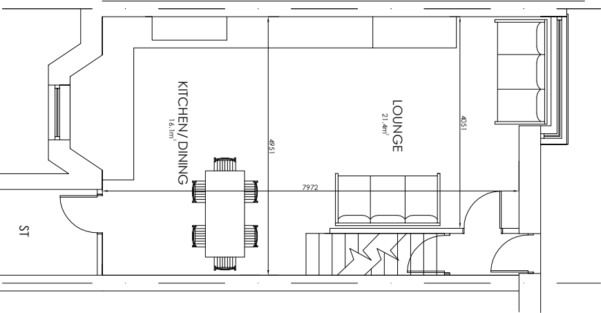
PROPOSED LOWER GROUND FLOOR PLAN
