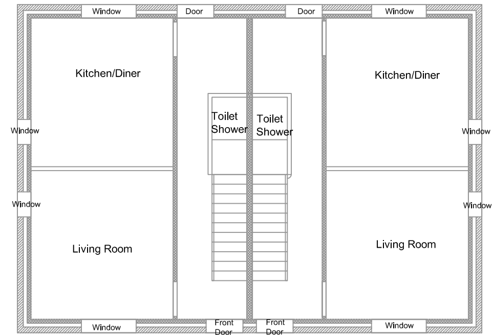
Semi-Detached Dwellings Ground Floor Layout
