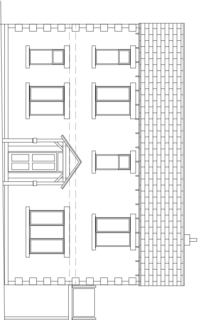
Front (South West) Elevation 1:100
