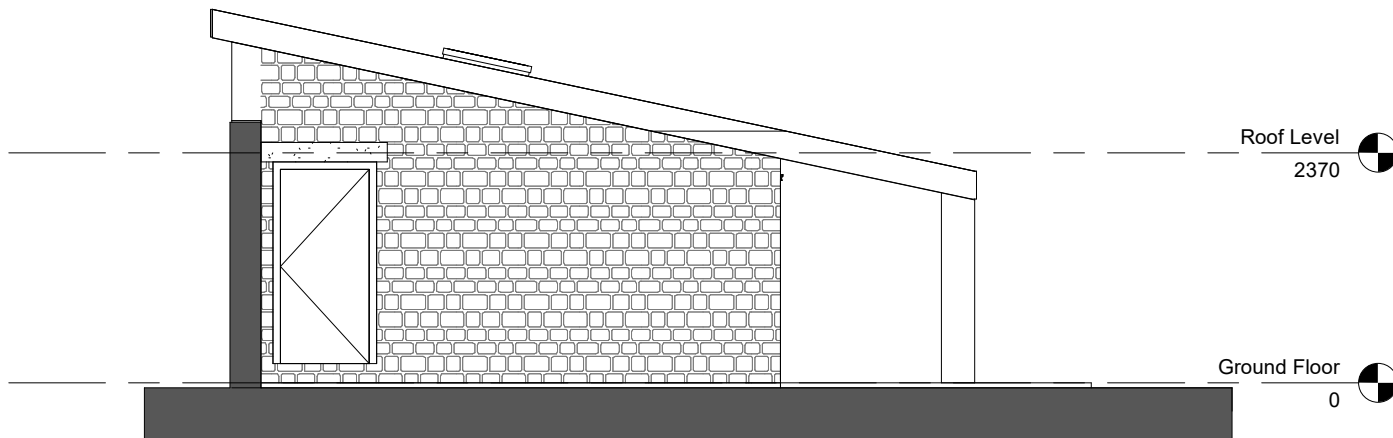
EXISTING SIDE ELEVATION 1 - 1/50
