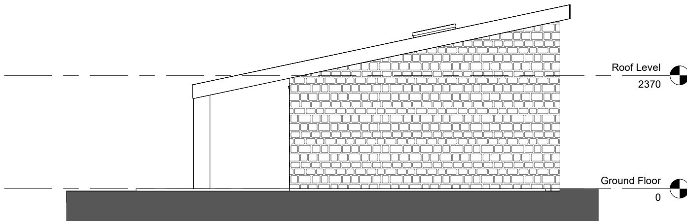
EXISTING SIDE ELEVATION 2 - 1/50
