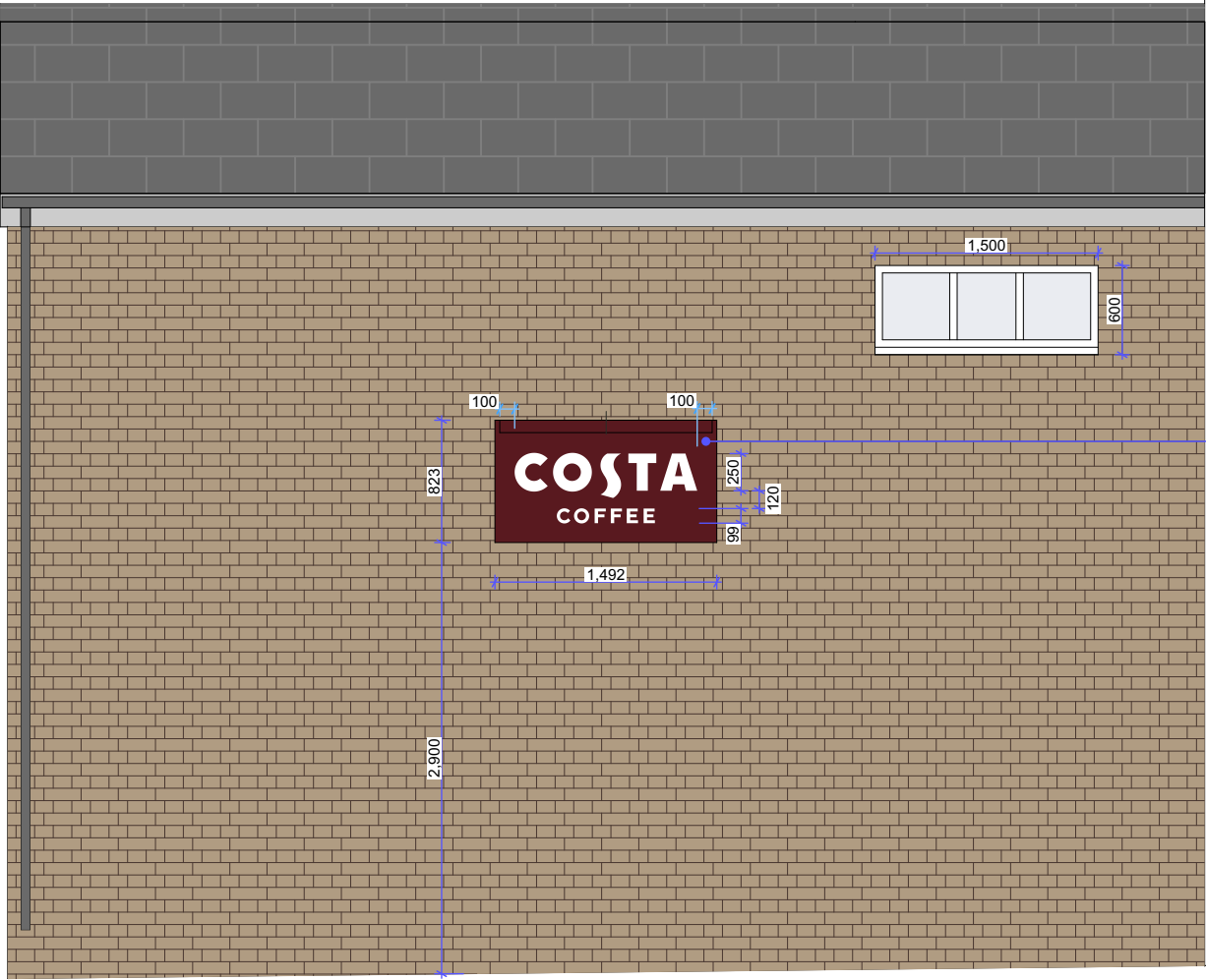
REAR ELEVATION
