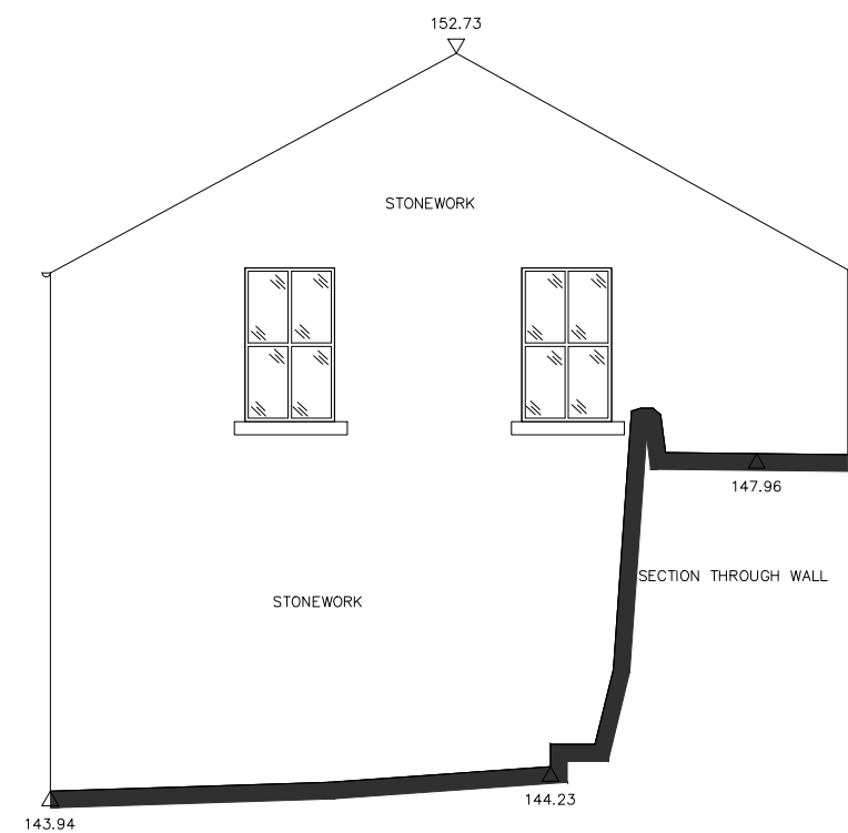
Datum 141.00m ELEVATION 2 (SOUTH ELEVATION)
