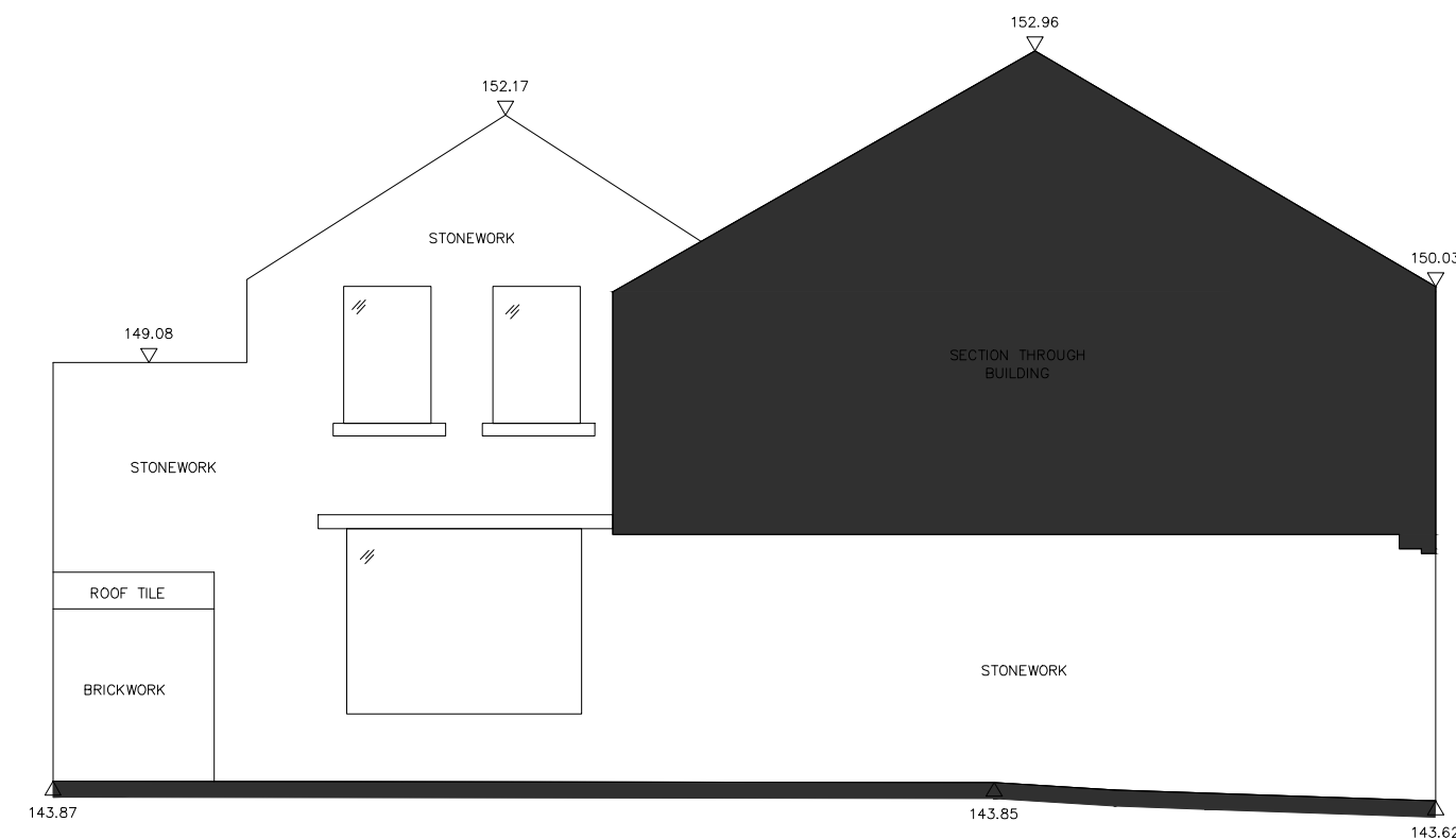
Datum 141.00m ELEVATION 5 (NORTH ELEVATION)
