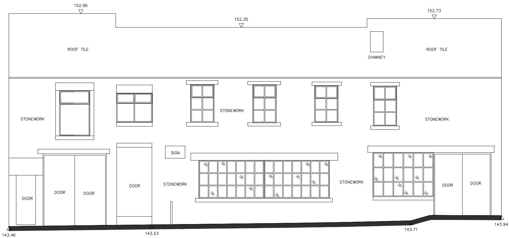
Datum 141.00m ELEVATION 1 (WEST ELEVATION)
