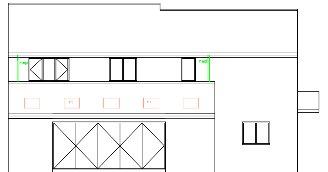
EXISTING REAR VIEW 1: 100
