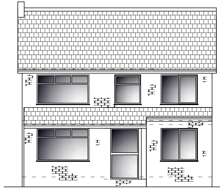
Front (East)
