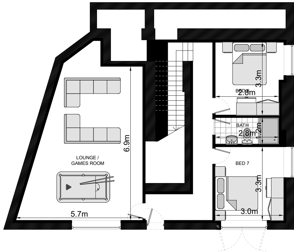
BASEMENT
