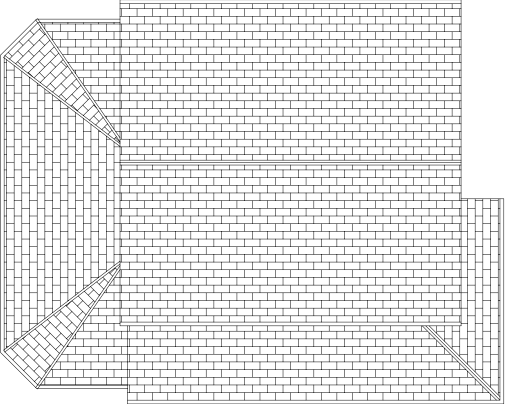
Existing Roof
