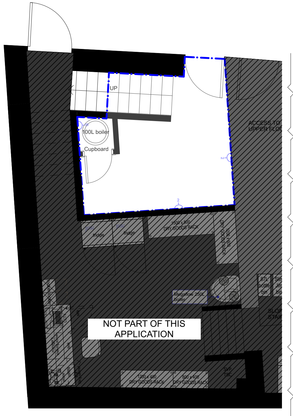
GROUND FLOOR
