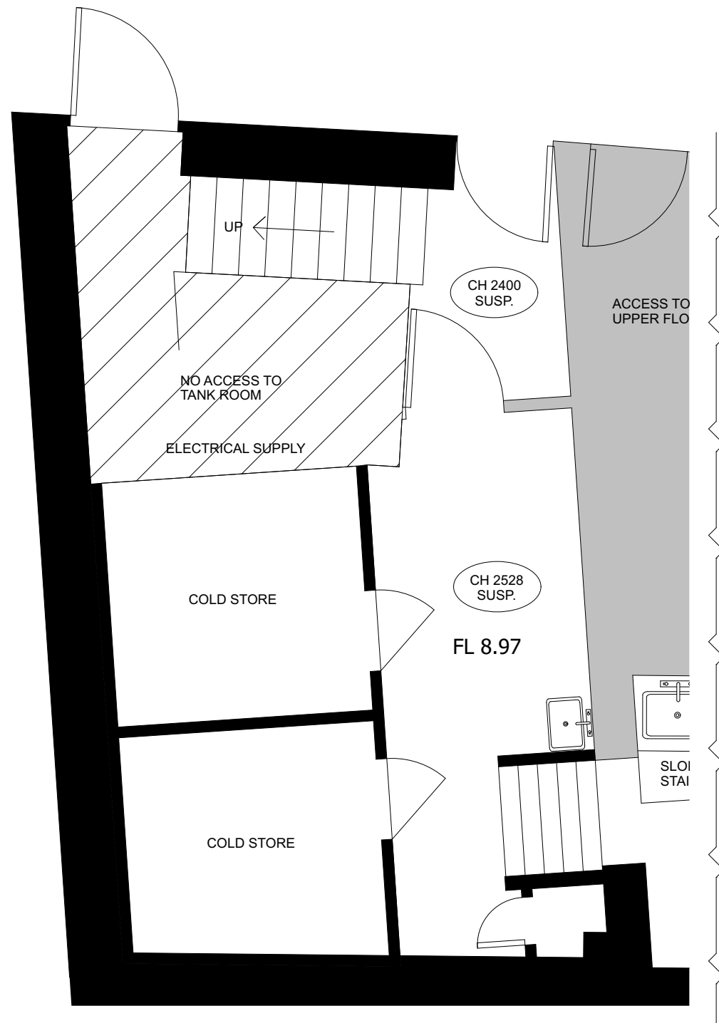
GROUND FLOOR
