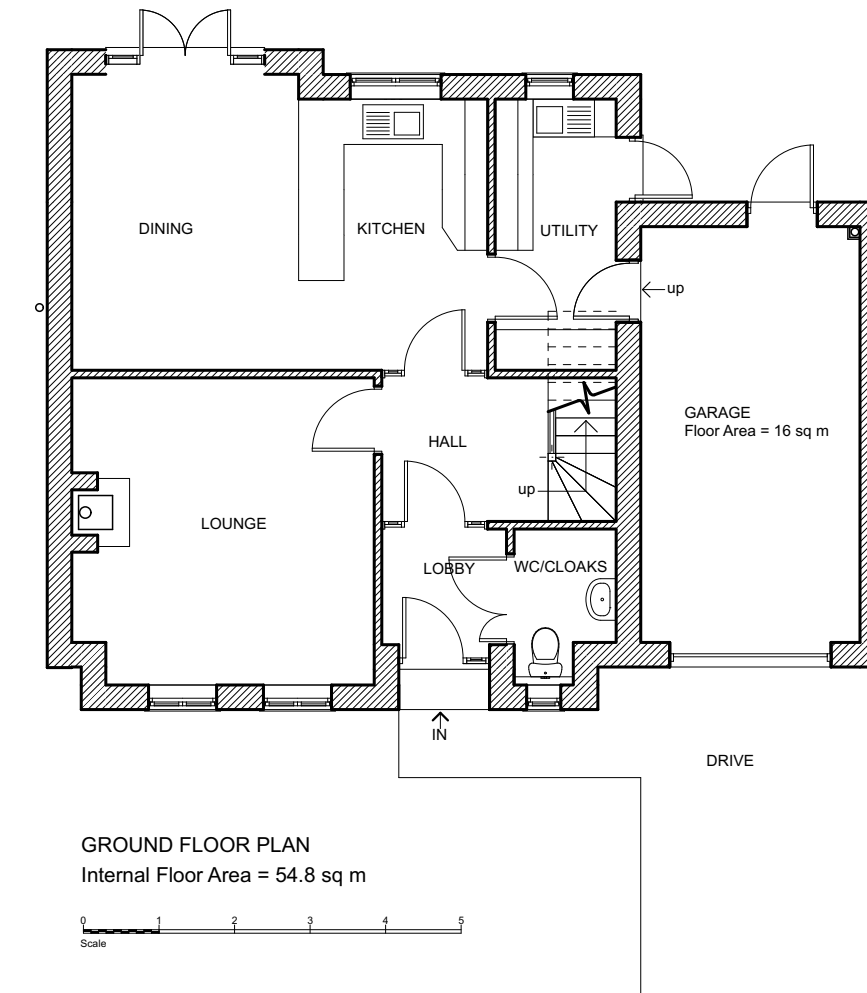
Ground Floor Plan - Plot 5
