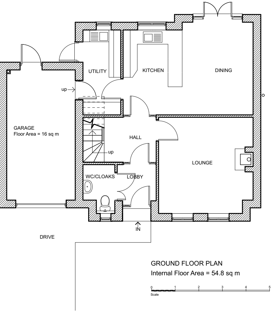
Ground Floor Plan - Plots 1-4
