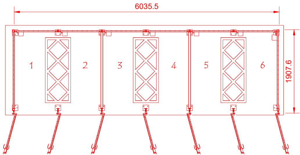
Floor Plan
