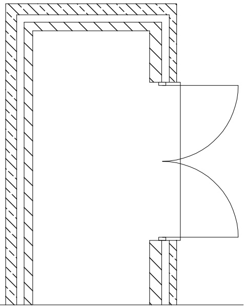
GARDEN ROOM AT BASEMENT LEVEL
