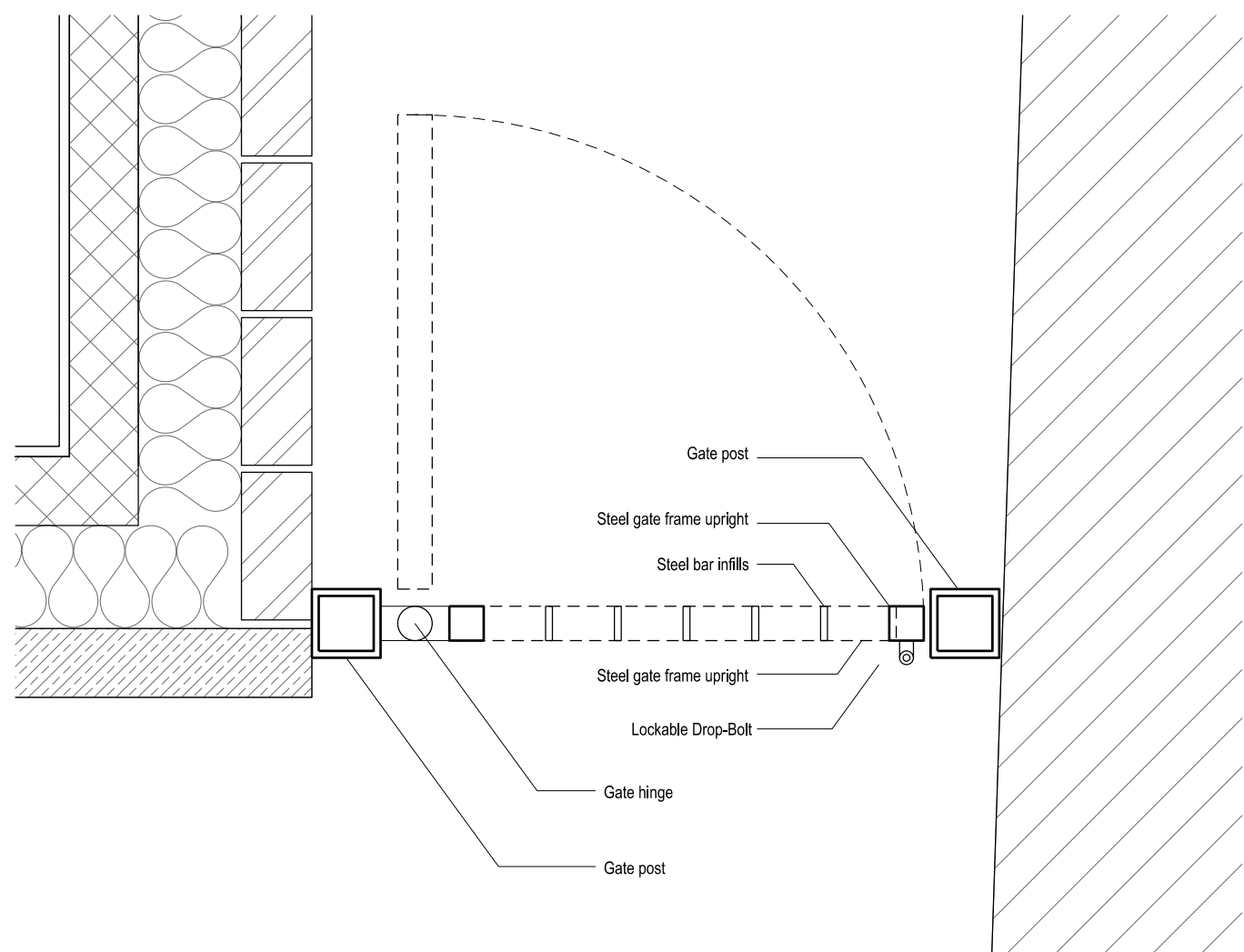
3 Plan Detail - Gate 03_11 1 : 10
