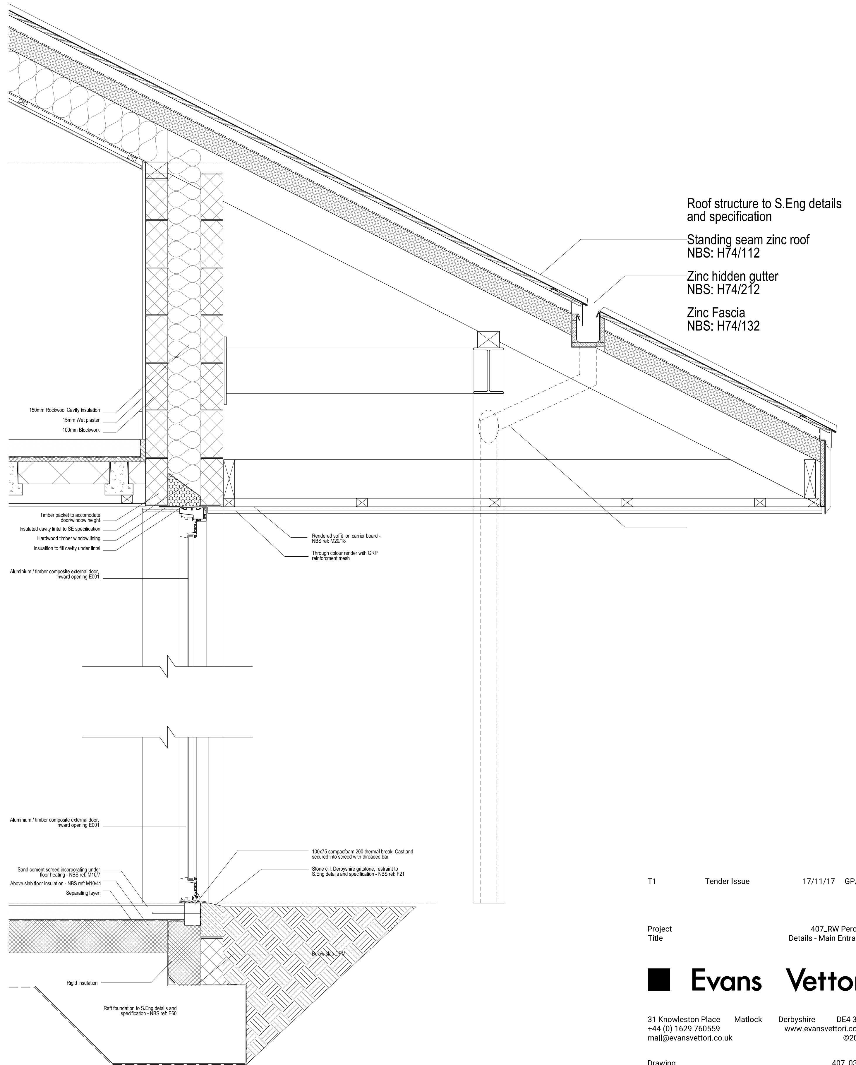
2 Section Detail - Main Entrance 03_11 1 : 10
