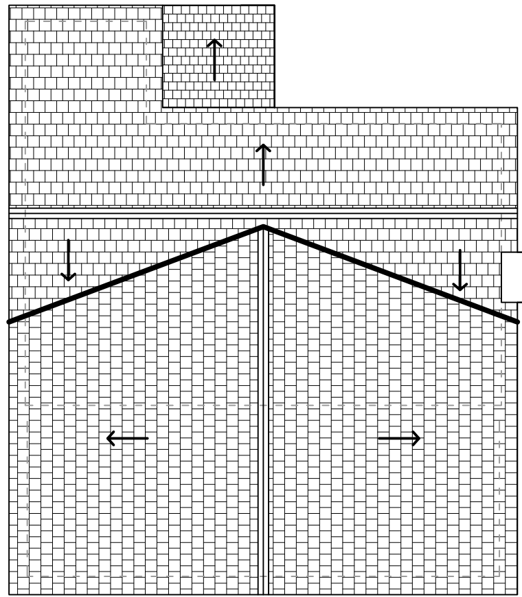
Roof Plan
