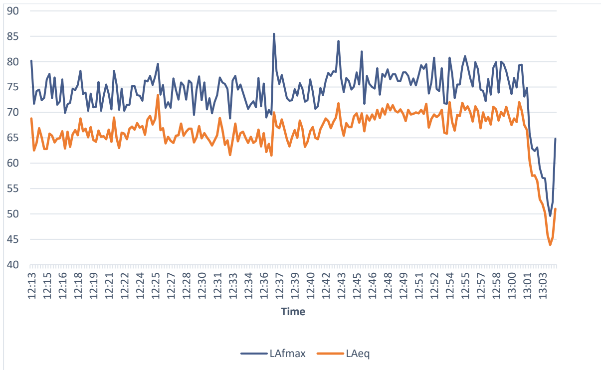
Environmental Noise Measurements, 28 th November 2017, Measurement M2
