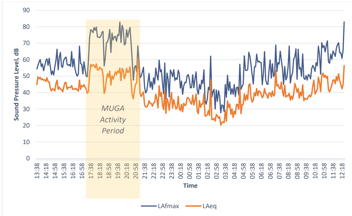
Environmental Noise Measurements, 8 th – 9 th August 2016, Measurement M1
