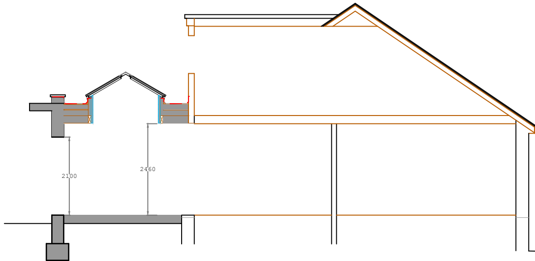
PROPOSED SECTION A-A
