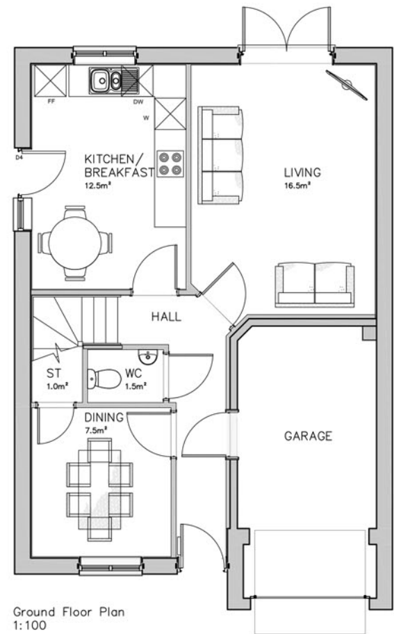
Ground Floor Plan 1:100 Total Floor Area 109.4m 2
